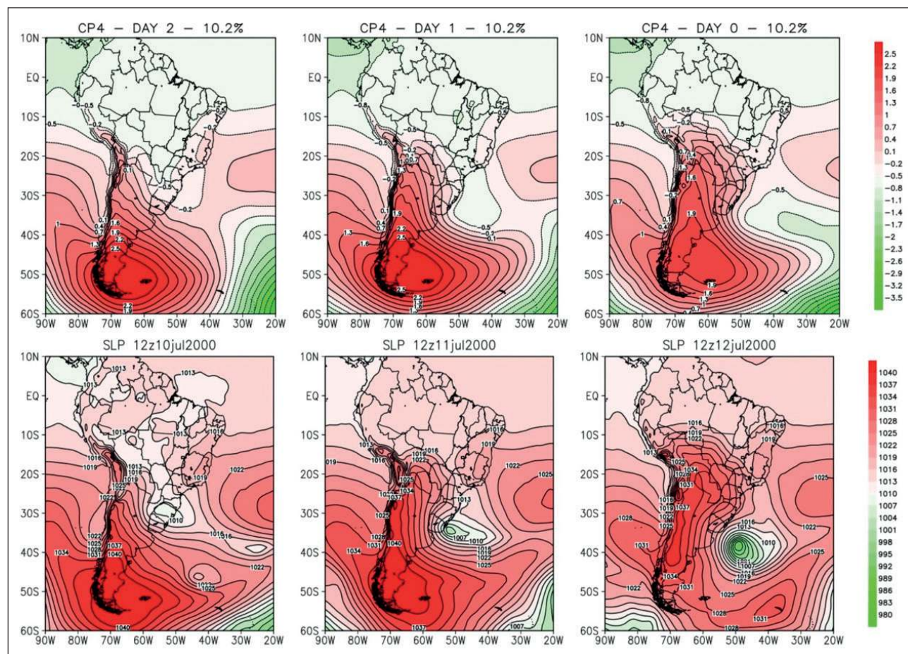
Figure 8 Top: fourth main sequence patterns (PSP4). Bottom: real sequence of Sea Level Pressure (SLP) fields for 10-12 July 2000 (Bottom).
