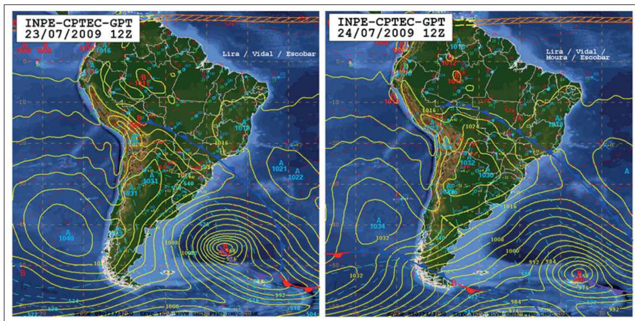
Figure 2 Surface synoptic charts from GPT/CPTEC at 12 Z: (left) 23 July 2009 and (right) 24 July/2009. Yellow lines represent the mean sea level pressure, red dashed lines are the layer thickness and the blue line indicates the cold fronts.
