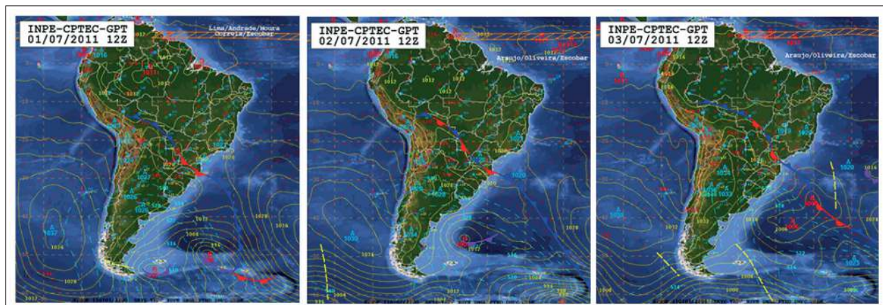
Figure 3 Surface synoptic charts elaborated by GPT/CPTEC at 12 Z. (left) 01 July 2011, (middle) 02 July 2011 and (right) 03 July 2011.
