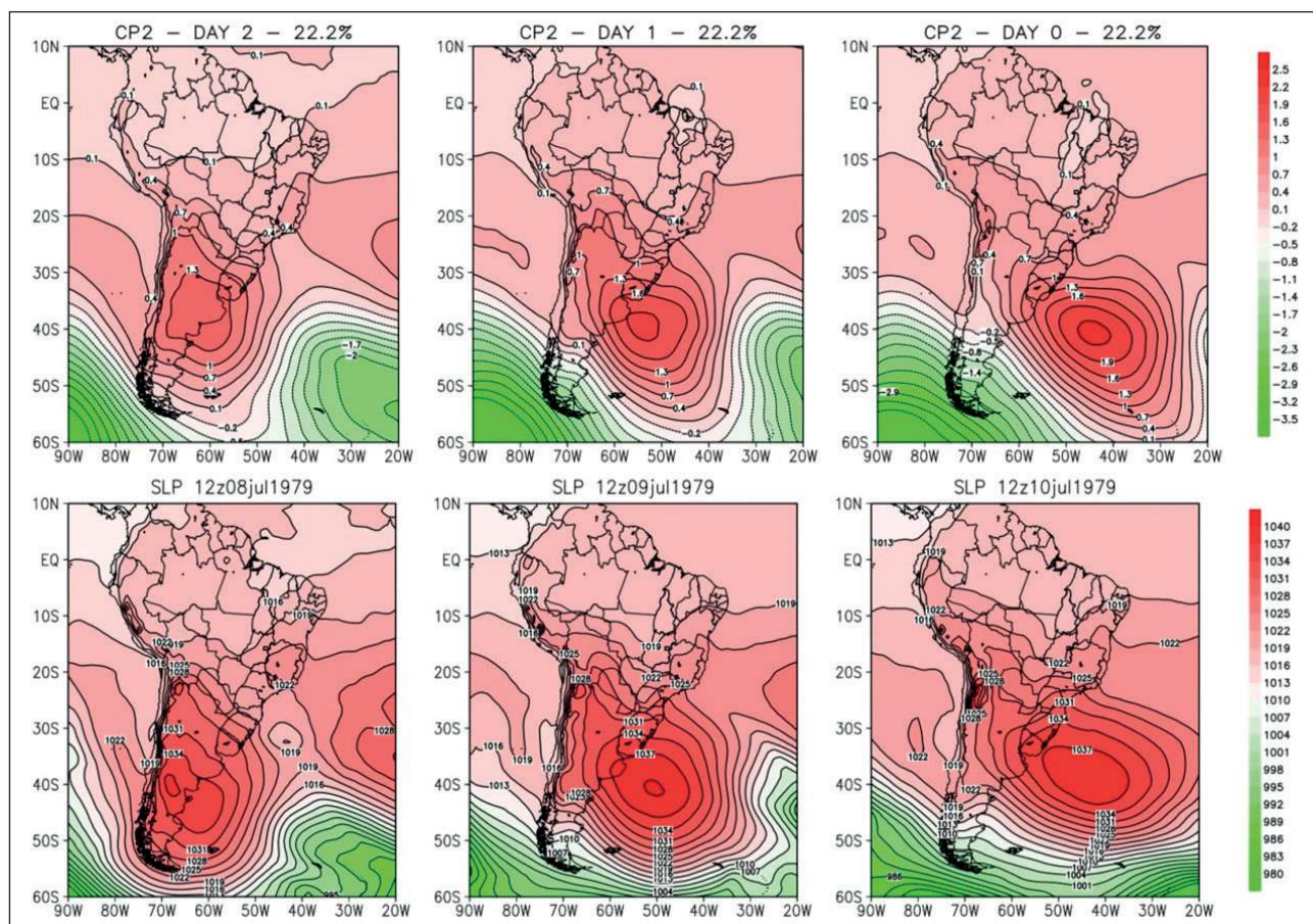
Figure 6 Top: second main sequence patterns (PSP2). Bottom: real sequence of Sea Level Pressure (SLP) fields for 8 July 1979 – 10 July 1979.
