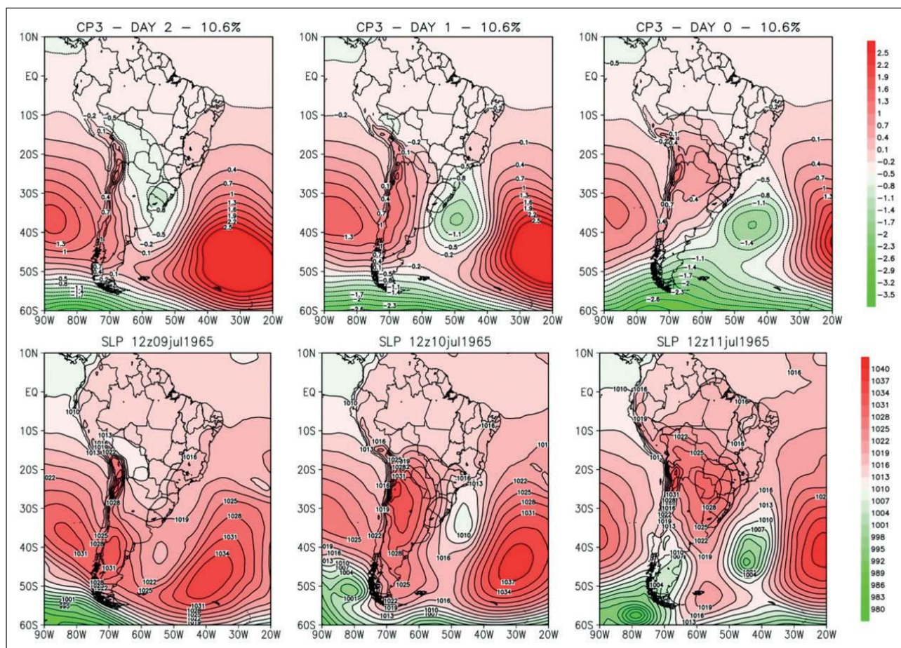
Figure 7 Top: third main sequence patterns (PSP3). Bottom: real sequence of Sea Level Pressure (SLP) fields for 9-11 July 1965 (Bottom).
