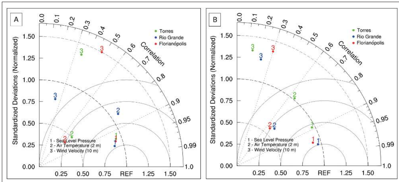
Figure 3 Taylor diagrams comparing the mean sea level pressure, air temperature and wind velocity of the simulation generated with the meteorological stations of Torres (green), Rio Grande (blue) and Florianópolis (Red); A. COA_EXP; and B. WRF_EXP.
