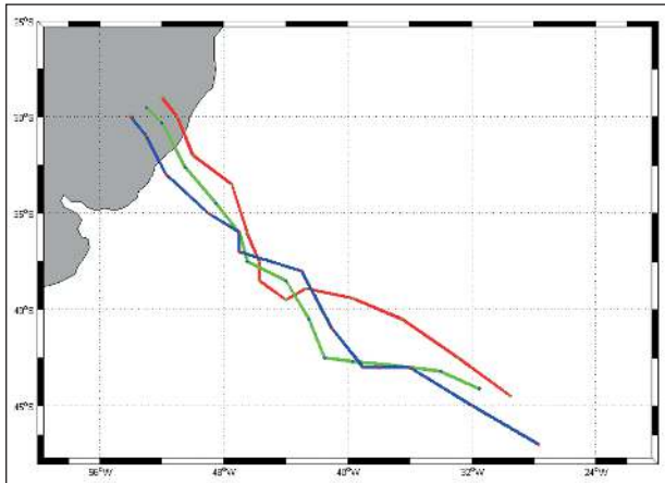
Figure 4 Extratropical cyclone trajectory extracted using minimum SLP data from COA_EXP (green line), WRF_EXP (red line) and CFSR (blue line) reanalysis.
