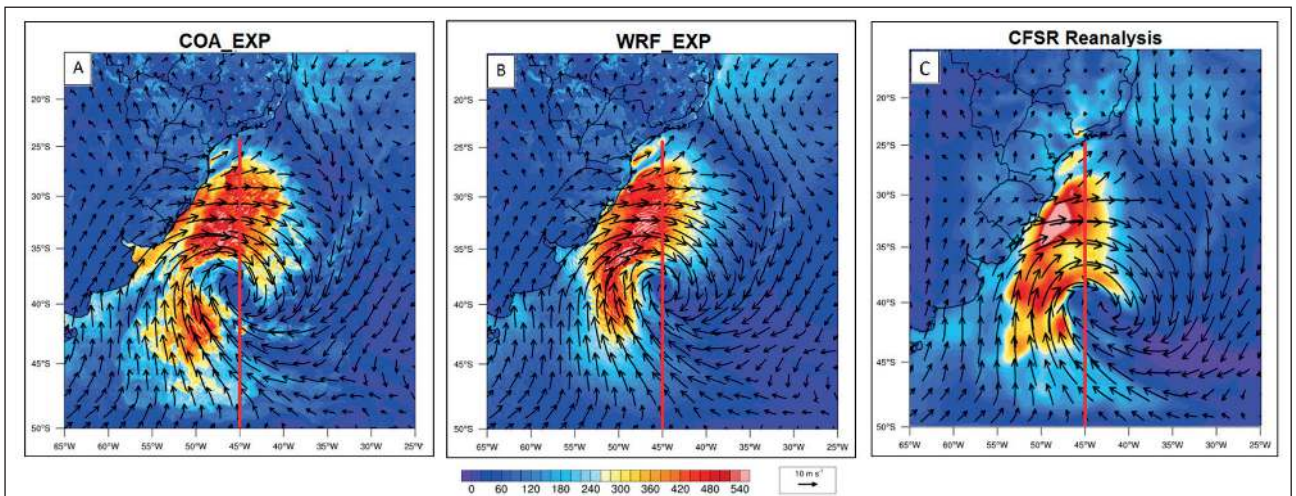
Figure 5 Latent Heat Flux ( \text{W m}^{-2} , shaded) and Wind Speed and Direction in 10 m ( \text{m s}^{-1} , vectors) for September 03 rd , 2006 at 1200 UTC. The section in red represents the longitudinal section at 45^{\circ}\text{W} shown in Figure 6. (A) COA_EXP (B) WRF_EXP (C) and CFSR database.
