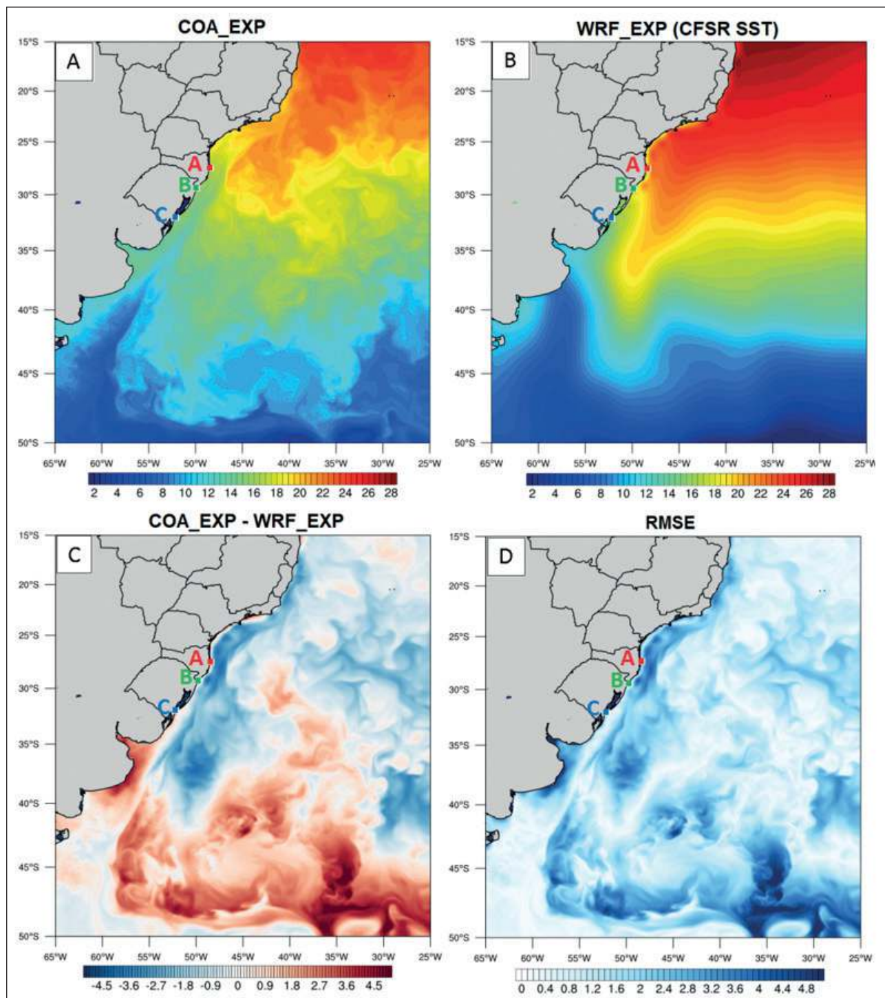
Figure 2 A. SST (°C) simulated by COA_EXP; B. SST (°C) from CFSR used in WRF; C. difference between SST (°C) simulated by COA_EXP and D. CFSR SST used in WRF_EXP RMSE between COA_EXP from SST (°C) and CFSR.
