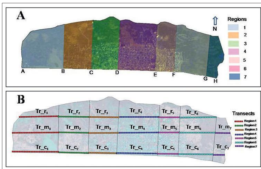
Figure 8 (A) Delimitation of the regions of the mask (A to H); (B) Transect locations per region, parallel to the coastline where Tr_{c(i)} , Tr_{m(i)} and Tr_{r(i)} indicate remote, intermediate and coastal transects, respectively and the subscript represents i-th region.
