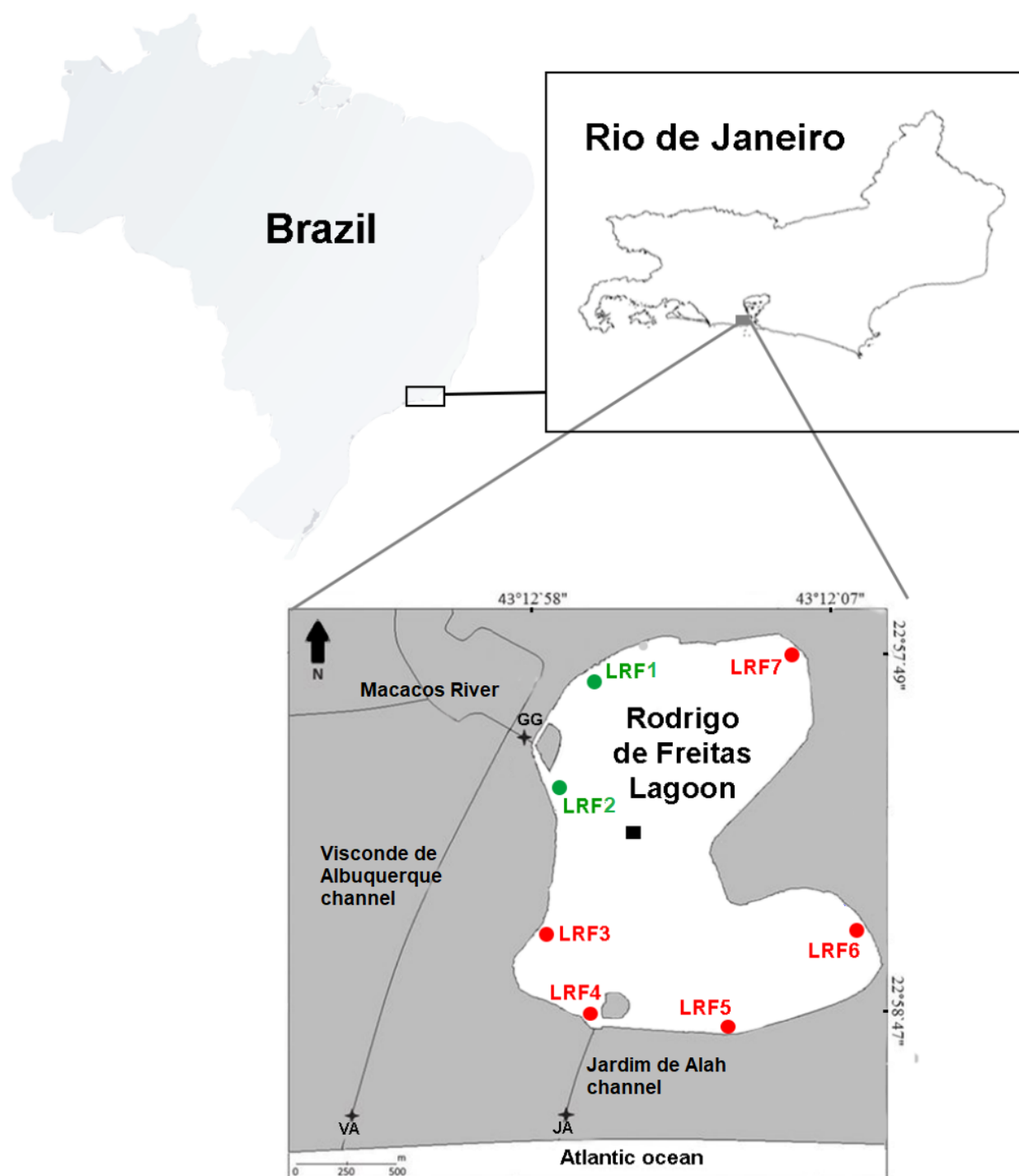
Figure 1. Location of the Rodrigo de Freitas Lagoon, Rio de Janeiro city, Southeastern Brazil. Sampling stations (LRF1-LRF7) and green color distinguish 1st week (●) sampling. The monitoring station of the municipal government is indicated by a square (■), and the location of artificial floodgates: GG General Garzon, VA Visconde de Albuquerque, and JA Jardim de Alah.
