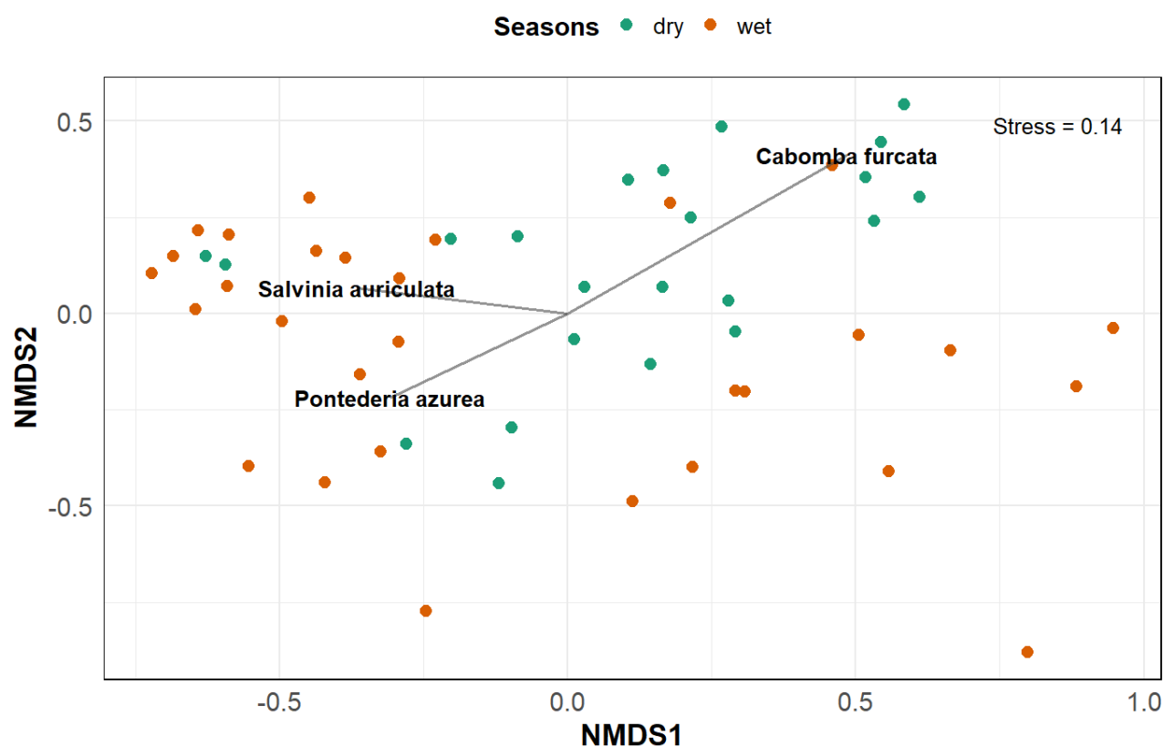
Figure 4. Non-metric multidimensional scaling (nMDS) ordination based on Bray-Curtis dissimilarities in macrophyte community composition per transect, showing seasonal variation between the wet and dry seasons at Ribeirão das Crioulas, Rio de Janeiro state, Brazil. Species vectors indicate the main contributors identified by SIMPER analysis. Stress value=0.14.
