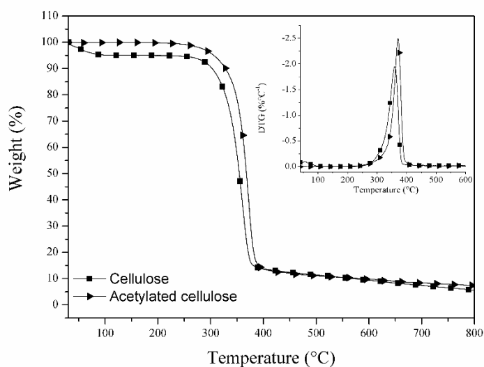
Figure 4: Thermogravimetric analyses of neat cellulose and acetylated cellulose.
