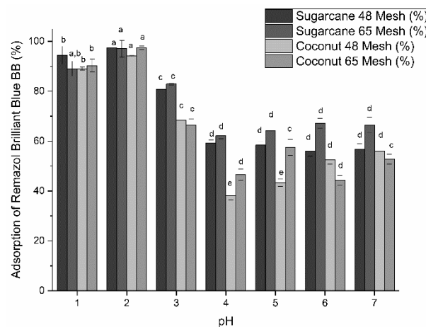
Figure 2: Effect of pH on adsorption of Remazol Brilliant Blue BB for sugarcane and coconut fibers with grit sizes of 48 and 65 Mesh. Means \pm standard deviation. Different letters indicate significant differences between the samples (Tukey test, p \leq 0.05 ). The test conditions included an adsorbent concentration of 50 g L -1 and an incubation of 12 hours for the sugarcane and 24 hours for the coconut fibers.
