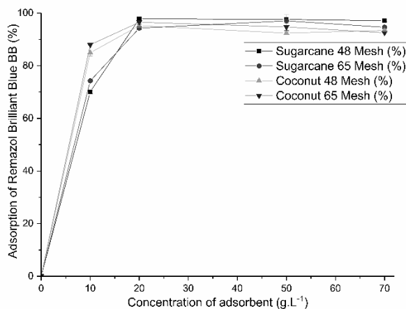
Figure 3: The effect of adsorbent concentration on the adsorption of the dye Remazol Brilliant Blue BB for sugarcane and coconut fibers with grit sizes of 48 and 65 Mesh. Means ± standard deviation. The test conditions included a time of contact of 12 hours for the sugarcane fiber and 24 hours for the coconut fiber and a pH of 2 for all samples.
