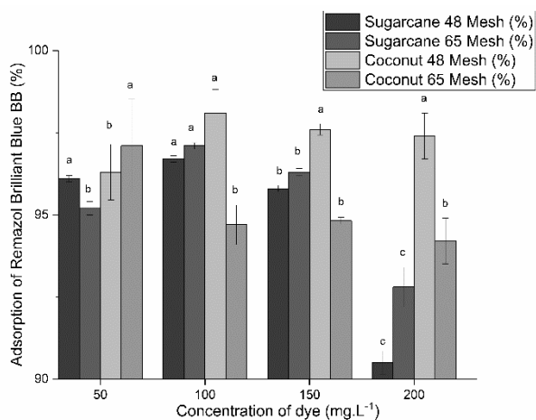
Figure 4: Effect of dye concentration on the adsorption of the dye Remazol Brilliant Blue BB for sugarcane and coconut fibers with grit sizes of 48 and 65 Mesh. Means \pm standard deviation. Different letters for the same dye concentrations indicate significant differences between the samples (Tukey test, p \leq 0.05 ). The test conditions were the time of contact of 12 hours for the sugarcane fiber and 24 hours for the coconut fiber, solution in pH of 2 and 20 g L -1 of fibers for all samples.
