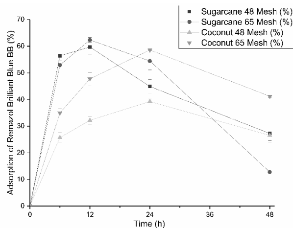
Figure 1: Effect of agitation time on the adsorption of the Remazol Brilliant Blue BB dye for sugarcane and coconut fibers with grit sizes of 48 and 65 Mesh. Mean \pm standard deviation. The test conditions were at the natural pH of the dye and the concentration of adsorbent 50 g.L -1 .
