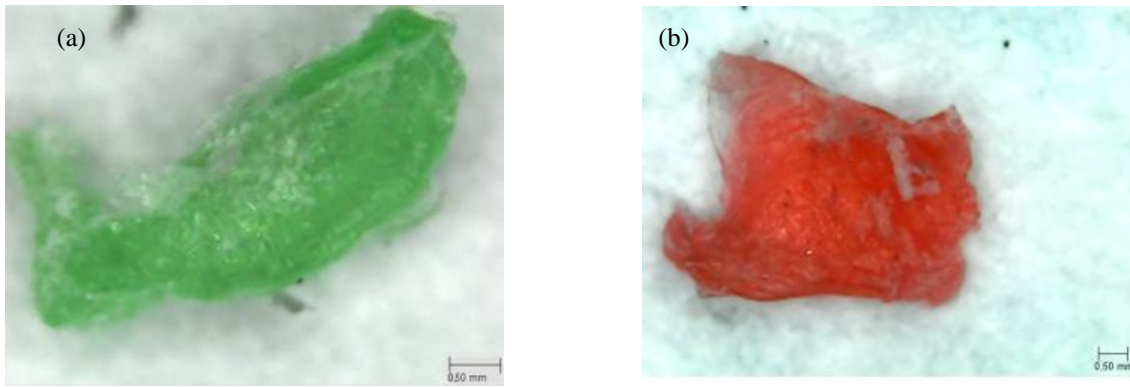
Figure 4: Images of cementitious matrix fracture surface with: a) PET and b) PP post-consumer flakes.
