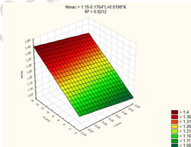
Figure 3: Surface graph of N_{mac} versus permeability and thickness.
